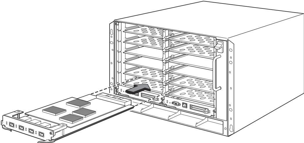
FIGURE 8 Installing a module in an 8-slot chassis
